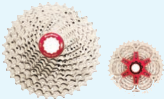
CSMX3113610 MX3 11-36T Alloy spider and locking Silver
